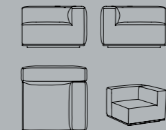
Right Arm W/D/H 105, 105, 67 CM SEAT HEIGHT 37 CM
