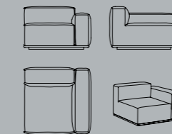
Corner W/D/H 105, 105, 67 CM SEAT HEIGHT 37 CM
