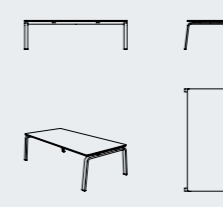
Man Coffee Table W/D/H 100, 48, 29 CM
