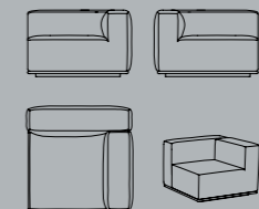
Right Arm W/D/H 105, 105, 67 CM SEAT HEIGHT 37 CM
