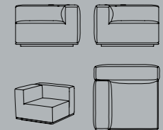
Center W/D/H 80, 105, 67 CM SEAT HEIGHT 37 CM
