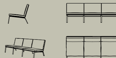
Man Three-Seater Sofa W/D/H 197, 74, 75 CM SEAT HEIGHT 37 CM
