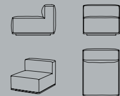
Left Arm W/D/H 105, 105, 67 CM SEAT HEIGHT 37 CM
