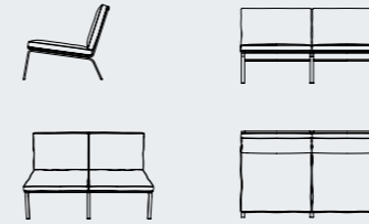
Man Two-Seater Sofa W/D/H 132, 74, 75 CM SEAT HEIGHT 37 CM
