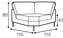
corner 90° no. 2
