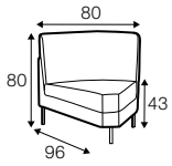
corner 30°
