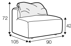
element 90 without armrests with back cushion 75x65
